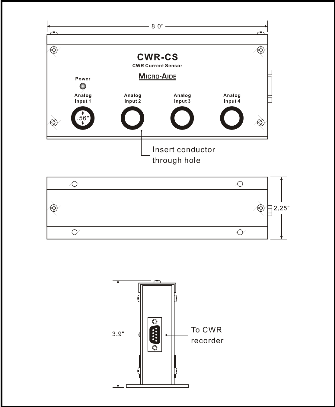
Figure 7 - CWR-CS Front, Top and Side Views
