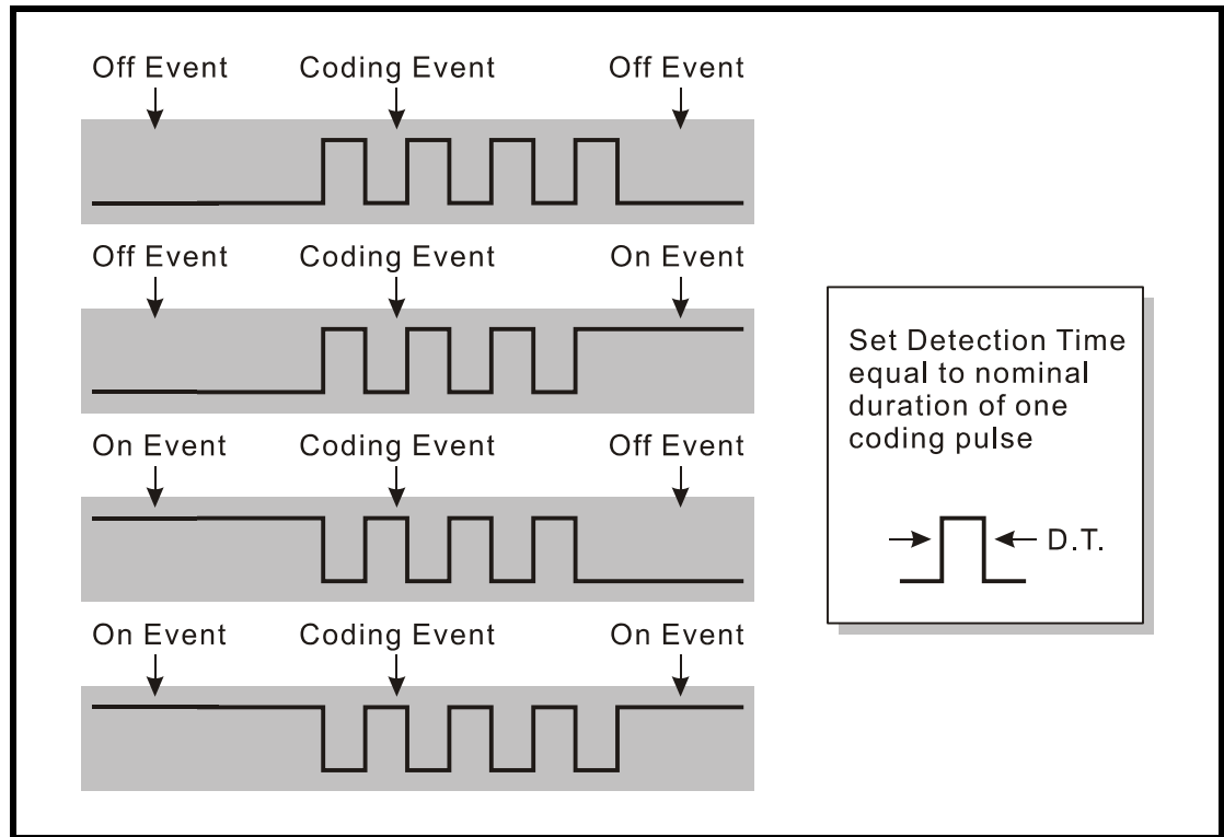
Figure 3 - Typical Code Signal Sequences
